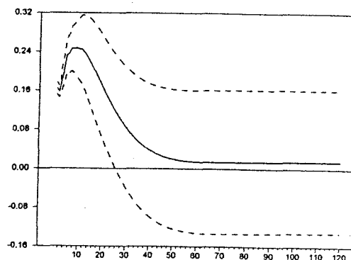
Figure 4. Response of unemployment to a transitory shock.
