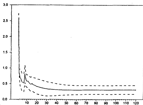
Figure 1. Response of inflation to a permanent shock.
