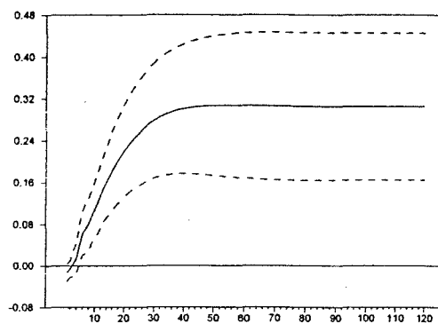
Figure 2. Response of unemployment to a permanent shock.
