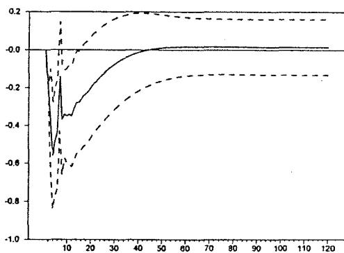
Figure 3. Response of inflation to a transitory shock.
